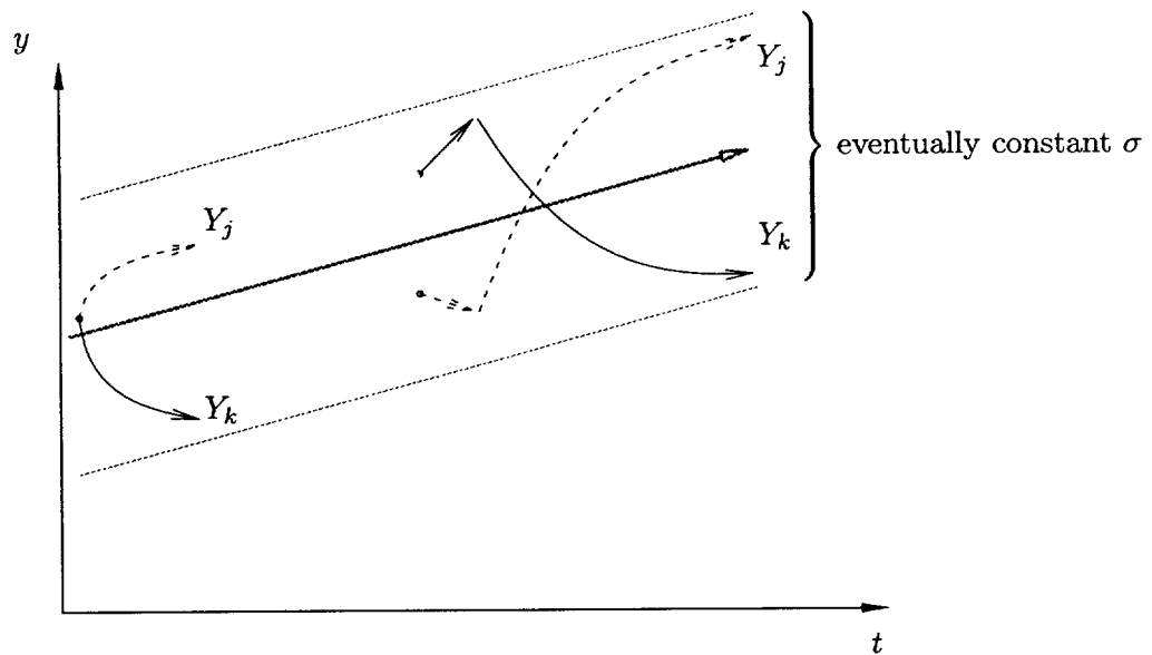
Fig. 10 (a): \sigma divergence towards \sigma -constant stationary state Figure shows a cross section of economies that begin close together relative to their steady state distribution and then spread out over time to converge in distribution to a well-defined steady state. Such dynamics are easy to generate, even with iid economies, each satisfying a covariance stationary linear autoregressive process.
