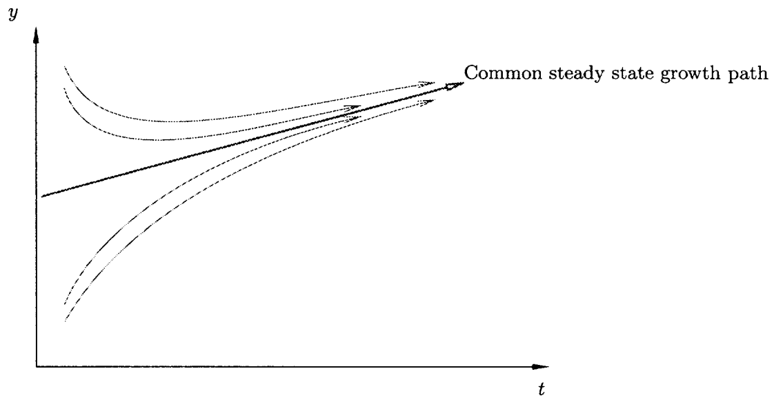
Fig. 10 (b): Coincident \beta and \sigma convergence Figure shows a cross section of economies where \beta and \sigma convergence coincide. All economies converge smoothly in towards the common steady state growth path. Similarly, the dispersion of the cross-section distribution declines to zero.
