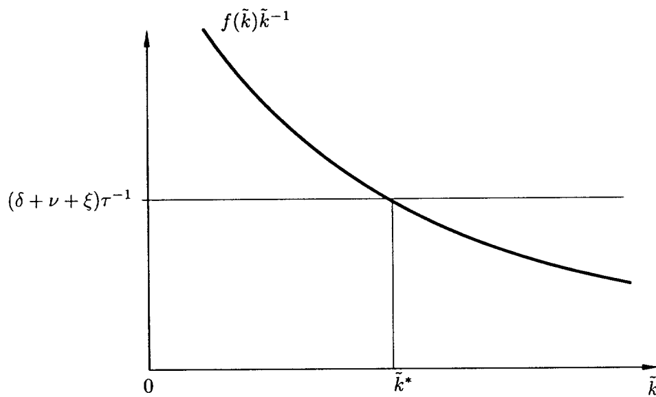
Fig. 2: Solow-Swan growth and convergence Function f(\tilde{k})\tilde{k}^{-1} is continuous, and tends to infinity and zero as \tilde{k} tends to zero and infinity respectively. Moreover, it is guaranteed to be monotone strictly decreasing. The vertical distance between f(\tilde{k})\tilde{k}^{-1} and (\delta + \nu + \xi)\tau^{-1} is \tau^{-1}\dot{\tilde{k}}/\tilde{k} . Convergence to steady state \tilde{k}^* therefore occurs for all initial values in \tilde{k} .
