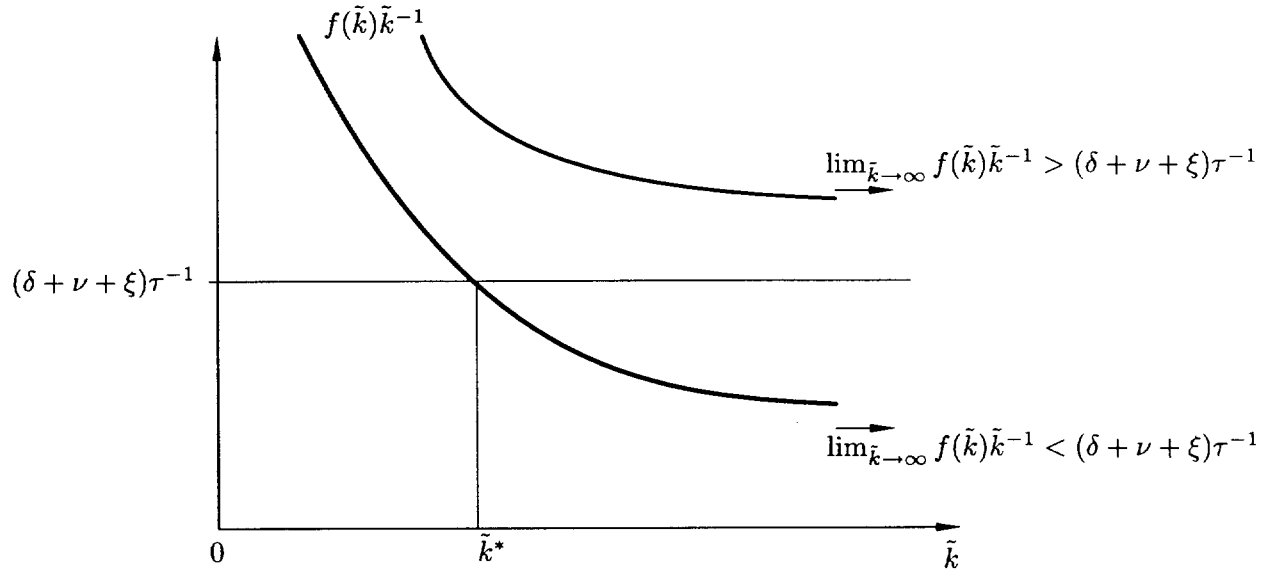
Fig. 5: Asymptotically linear ( O(\tilde{k}) ) growth and convergence The continuous function f(\tilde{k})\tilde{k}^{-1} tends to infinity as \tilde{k} tends to zero and to \lim_{\tilde{k} \rightarrow \infty} f(\tilde{k})\tilde{k}^{-1} > 0 as \tilde{k} tends to infinity. Moreover, it is guaranteed to be monotone strictly decreasing for finite \tilde{k} . The vertical distance between f(\tilde{k})\tilde{k}^{-1} and (\delta + \nu + \xi)\tau^{-1} is \tau^{-1}\dot{\tilde{k}}/\tilde{k} . If \lim_{\tilde{k} \rightarrow \infty} f(\tilde{k})\tilde{k}^{-1} < (\delta + \nu + \xi)\tau^{-1} then convergence occurs as in the Solow-Swan model with some constant finite \tilde{k}^* describing balanced-growth equilibrium. However, if \lim_{\tilde{k} \rightarrow \infty} f(\tilde{k})\tilde{k}^{-1} > (\delta + \nu + \xi)\tau^{-1} then \dot{\tilde{k}}/\tilde{k} is always positive, and balanced growth obtains only as \tilde{k} \nearrow \infty . Every initial \tilde{k}(0) is part of an equilibrium tending towards balanced growth.
