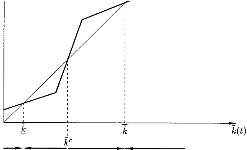
Fig. 7: Multiple locally stable steady states Either of the two possible limit points \bar{k} or \tilde{\bar{k}} obtains, depending on \tilde{k}(0) \gtrless \tilde{k}^c . The dark kinked line describes \tilde{k}(t+1) as a function of \tilde{k}(t) in the Galor-Zeira model, as applied in Quah [92] to study economies confronting imperfect capital markets. If a cross section of economies had randomly distributed initial conditions \tilde{k}(0) , then over time the cross-section distribution of \tilde{k} 's (and thus of \tilde{y} 's) will tend towards a clustering around \bar{k} and \tilde{\bar{k}} .
