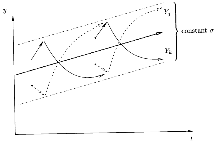
Fig. 10 (c): \sigma convergent limit with ongoing intra-distribution churning Figure shows a cross section of economies at the steady-state distribution limit, but displaying ongoing intra-distribution dynamics. This situation might be viewed as the distributional endpoint of the earlier Fig. 10 (a).
