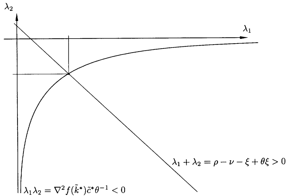
Fig. 3: Eigenvalues in the Cass-Koopmans model Since \nabla^2 f(\bar{k}^*)\bar{c}^*\theta^{-1} = \left(\nabla^2 f(\bar{k}^*)\bar{k}^*\right) \left[f(\bar{k}^*)/\bar{k}^* - (\delta + \nu + \xi)\right] \theta^{-1} , if f(\bar{k}) = \bar{k}^\alpha , with \alpha \in (0, 1) then as \alpha increases towards unity the negative eigenvalue \lambda_2 rises towards zero.
