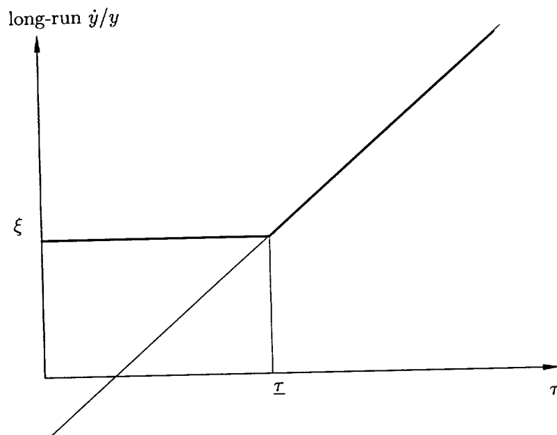
Fig. 6: Threshold effect of savings on long-run income growth rates in O(k) model For economies with savings rates \tau less than the threshold value \underline{\tau} , the long-run income growth rate is \xi independent of \tau . If \tau > \underline{\tau} , however, then savings rates positively affect long-run growth.
