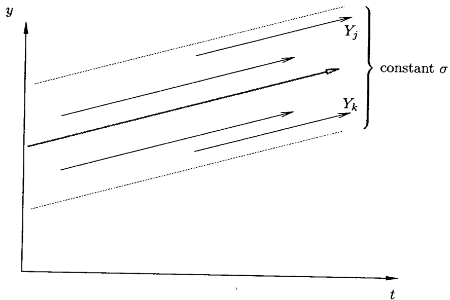
Fig. 10 (d): \sigma -convergent limit without intra-distribution churning Figure shows a cross section of economies at the steady-state distribution limit, but unlike in Fig. 10 (c) there are no ongoing intra-distribution dynamics. All economies simply move in parallel.
