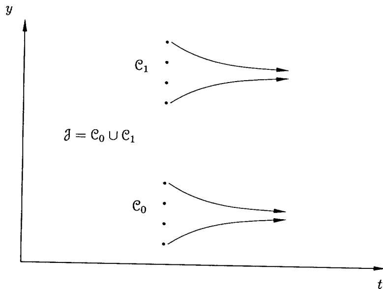
Fig. 9: Distinct average \mathbf{H} across clubs Each economy now has a natural clustering—either C_0 or C_1 again with J the entire cross section—so that the relevant average \mathbf{H} differs across economies. As drawn here convergence occurs to a two-point or twin-peaked distribution.
